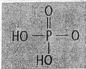
Phosphate group
