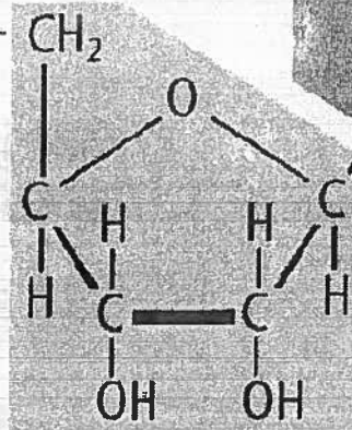
Sugar
