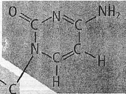
Nitrogen-containing base
